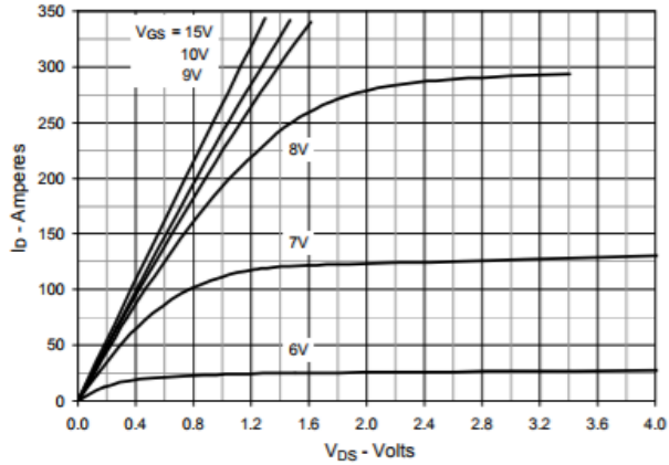
Fig. 1. Extended Output Characteristics @ T_J = 25^\circ\text{C}
