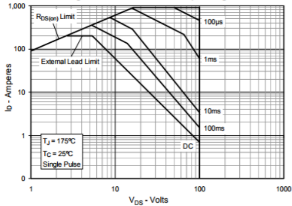
Fig. 11. Forward-Bias Safe Operating Area
