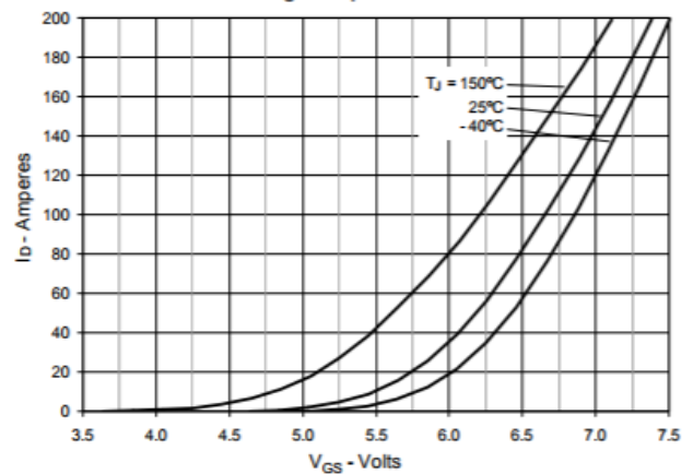
Fig. 6. Input Admittance
