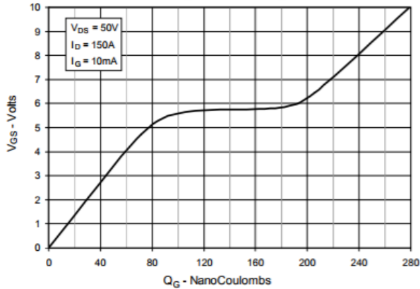
Fig. 9. Gate Charge
