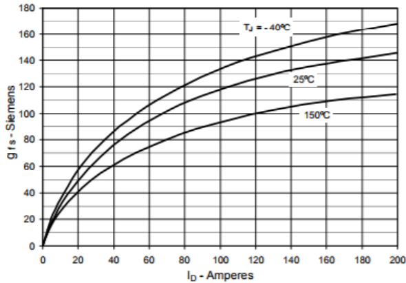
Fig. 7. Transconductance
