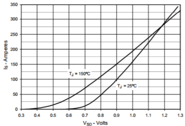
Fig. 8. Forward Voltage Drop of Intrinsic Diode
