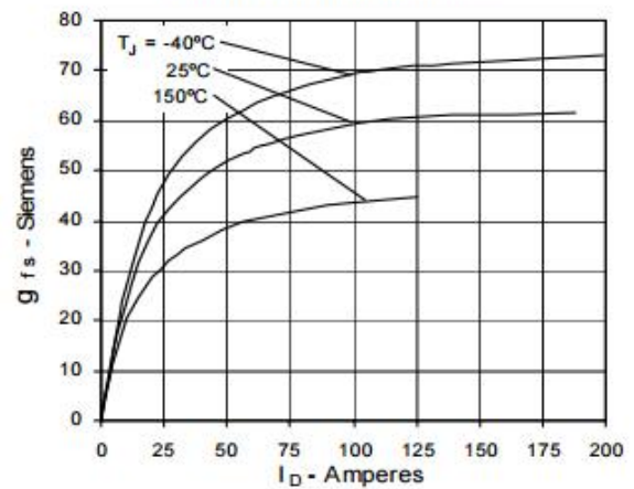
Fig. 8. Transconductance
