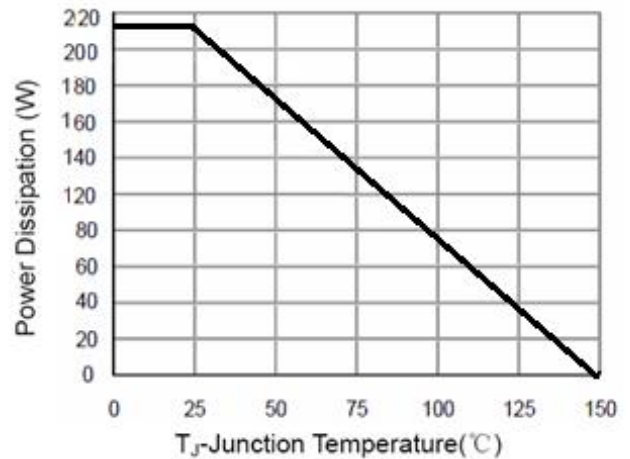
Figure 9 Power De-rating
