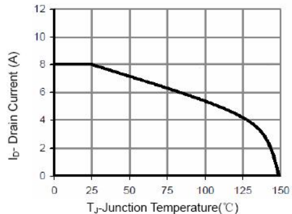
Figure 9 Current De-rating
