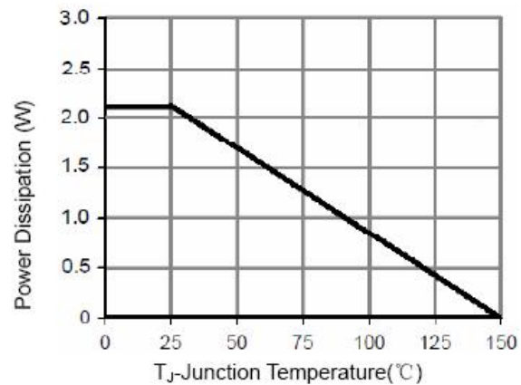
Figure 10 Power De-rating
