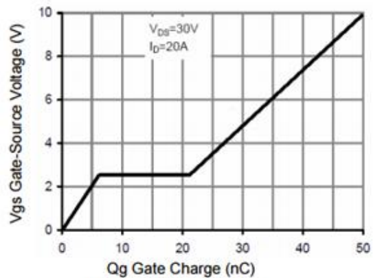
Figure 5 Gate Charge
