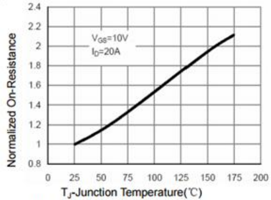
Figure 4 Rdson-Junction Temperature
