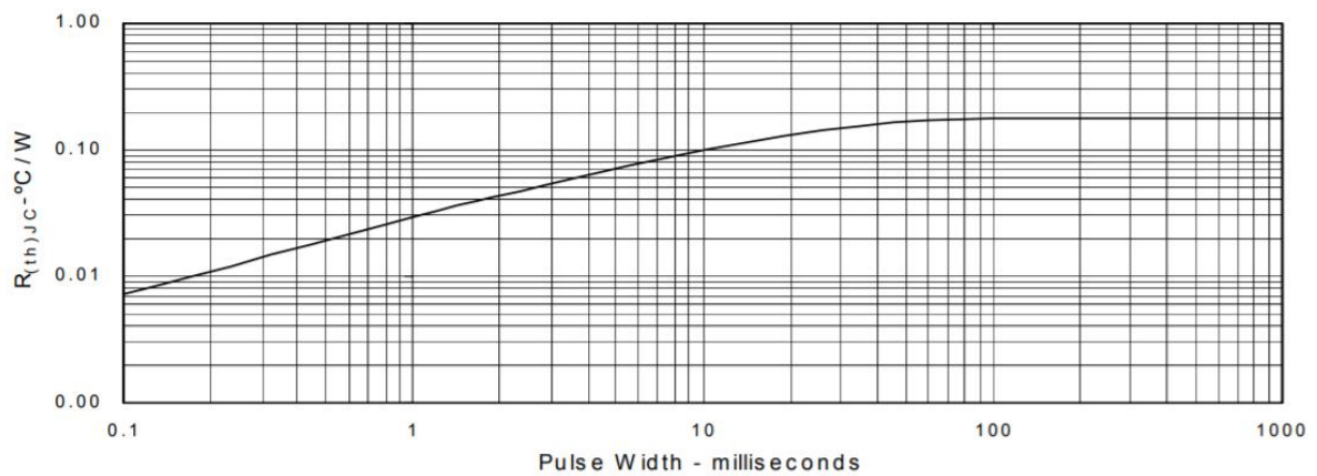
Fig. 13. Maximum Transient Thermal Resistance
