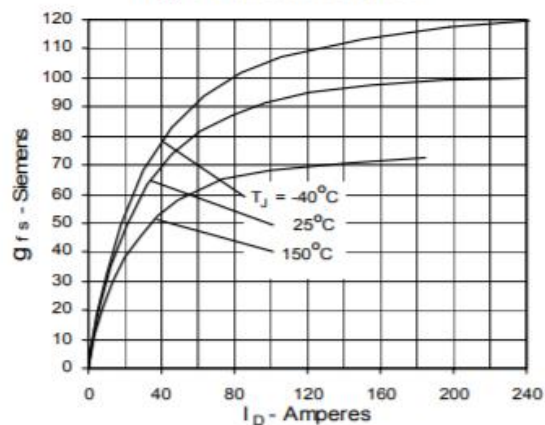
Fig. 8. Transconductance
