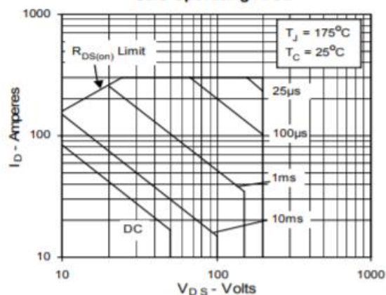
Fig. 12. Forward-Bias Safe Operating Area
