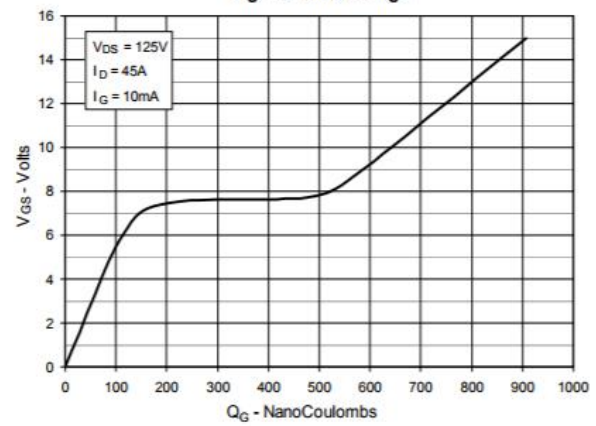
Fig. 10. Gate Charge
