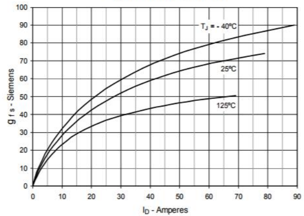
Fig. 8. Transconductance
