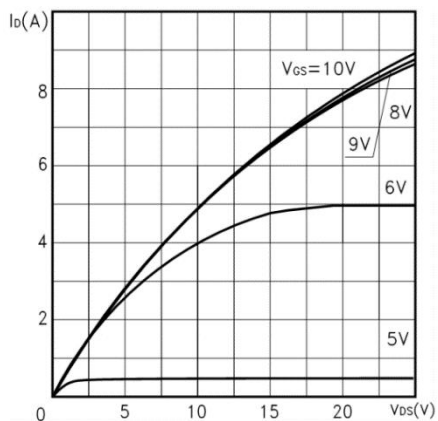
Figure 3. Output characteristics
