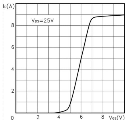
Figure 4. Transfer characteristics
