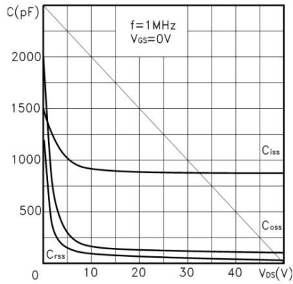
Figure 7. Capacitance variations
