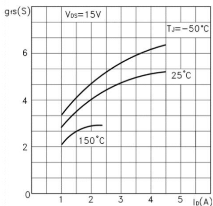
Figure 5. Transconductance
