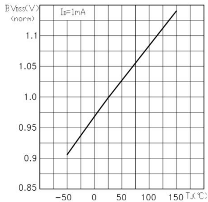
Figure 11. Normalized BV_{DSS} vs temperature
