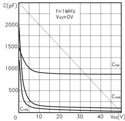
Figure 7. Capacitance variations
