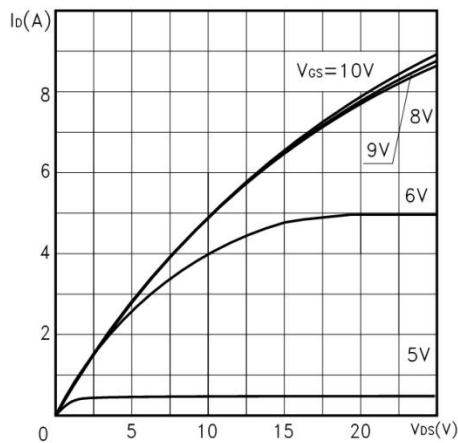
Figure 3. Output characteristics
