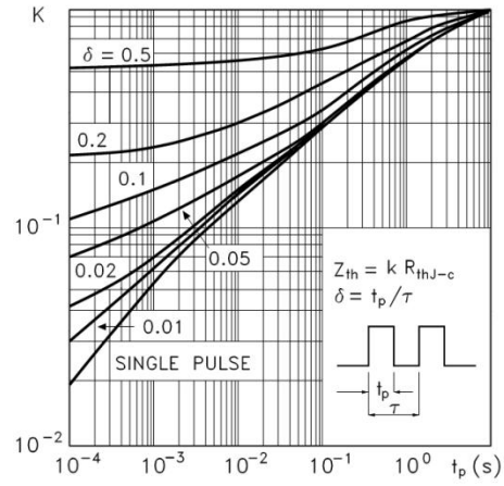
Figure 2. Thermal impedance
