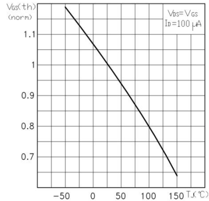
Figure 8. Normalized gate threshold voltage vs temperature
