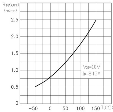
Figure 9. Normalized on resistance vs temperature
