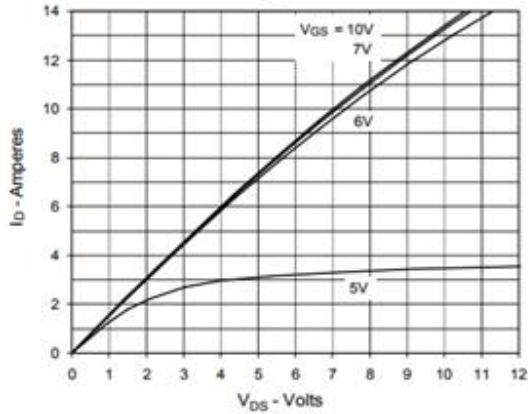
Fig. 1. Output Characteristics @ 25°C
