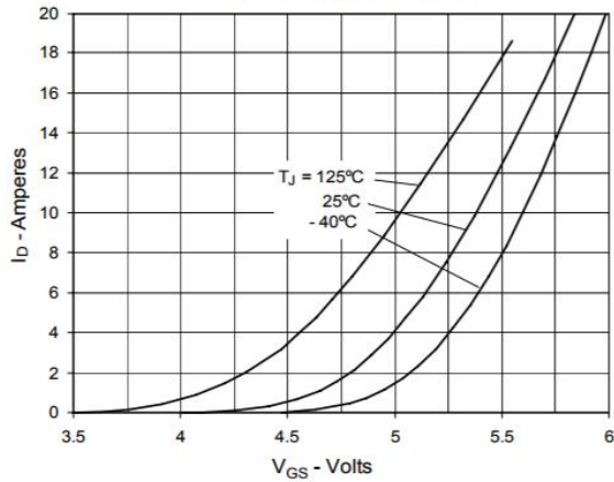
Fig. 7. Input Admittance
