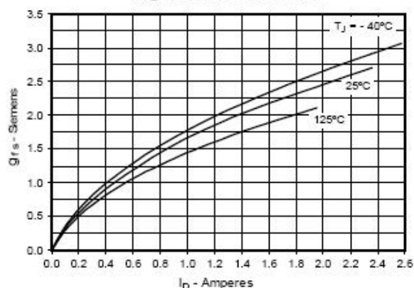
Fig. 8. Transconductance
