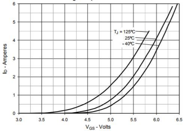
Fig. 7. Input Admittance
