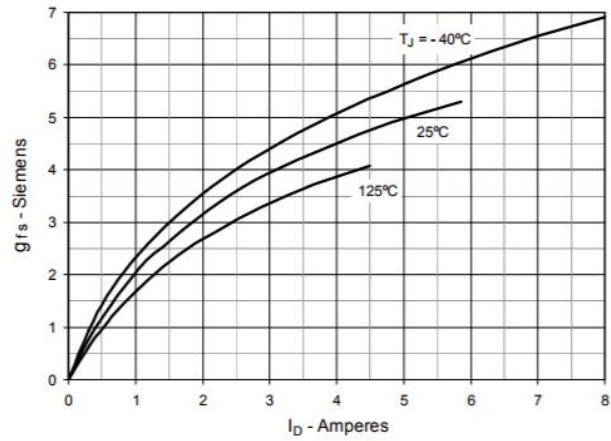
Fig. 8. Transconductance
