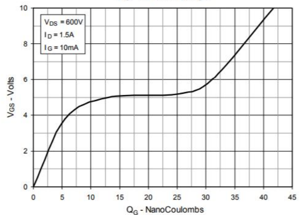
Fig. 10. Gate Charge
