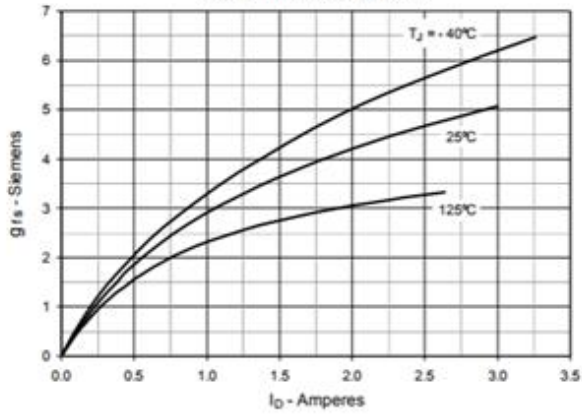
Fig. 7. Transconductance
