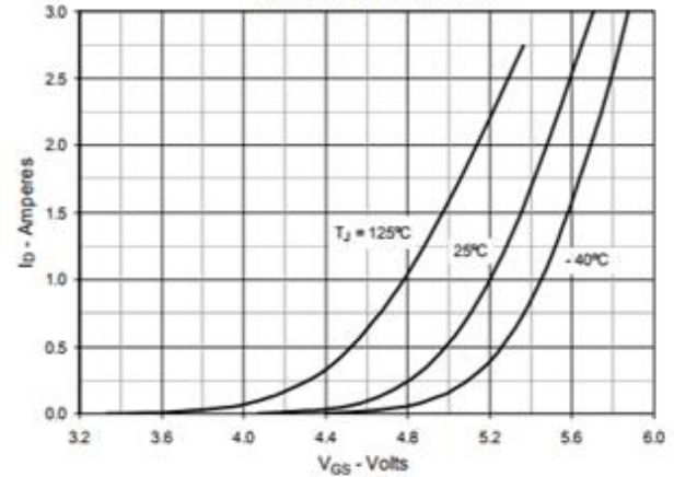
Fig. 6. Input Admittance
