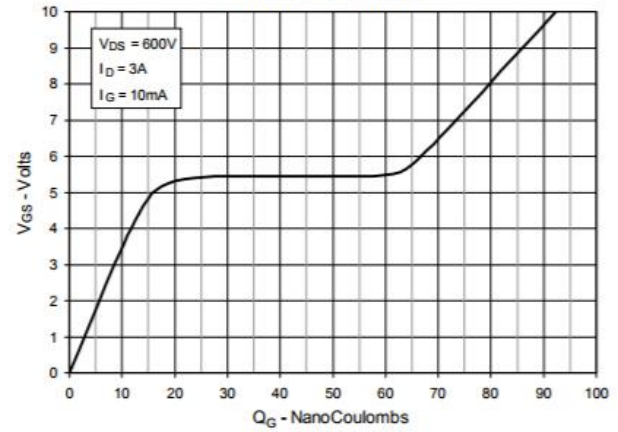
Fig. 10. Gate Charge
