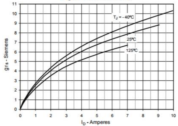
Fig. 8. Transconductance
