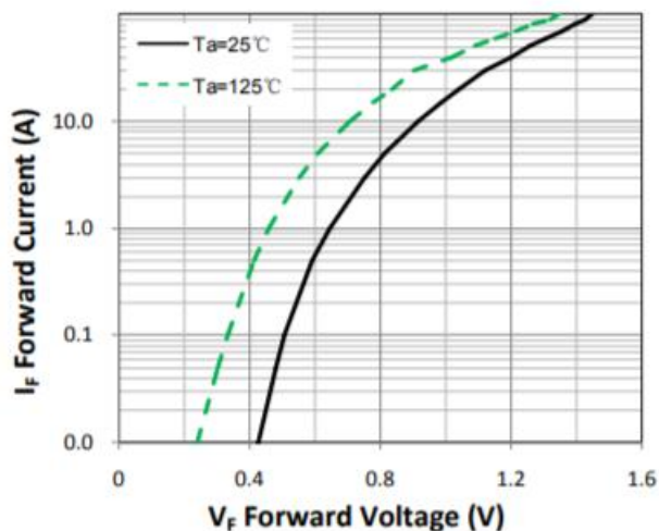
Figure 1. Forward Characteristic(typ.)
