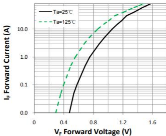
Figure 1. Forward Characteristic(typ.)
