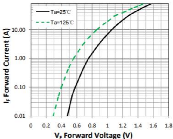
Figure 1. Forward Characteristic(typ.)
