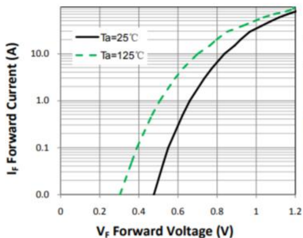
Figure 1. Forward Characteristic(typ.)
