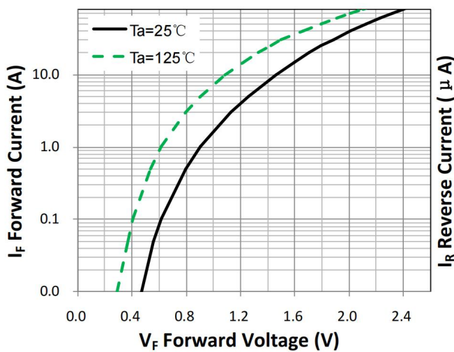
Figure 1. Forward Characteristic(typ.)
