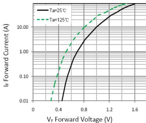
Figure 1. Forward Characteristic(typ.)
