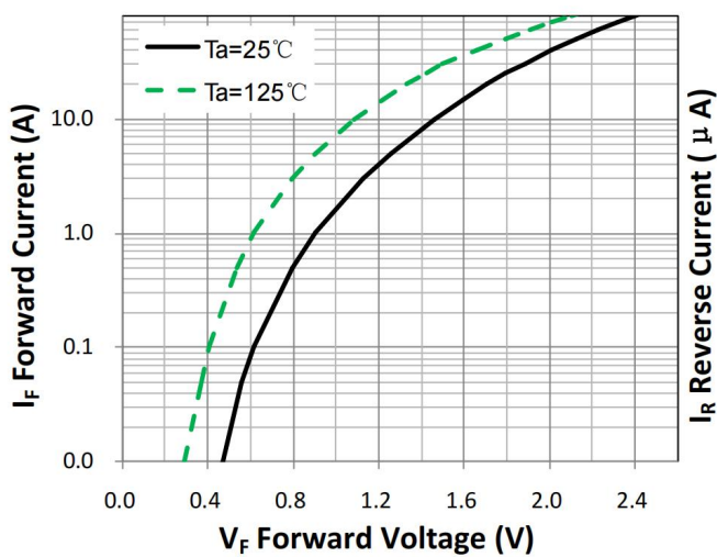
Figure 1. Forward Characteristic(typ.)
